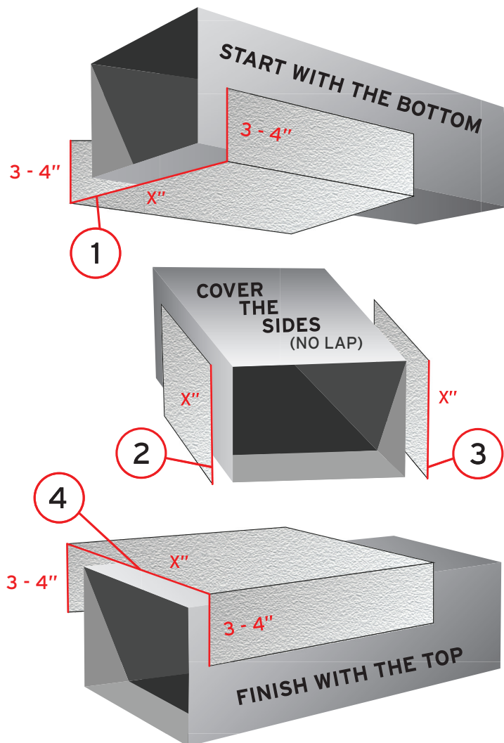
Peel back the width of your lap by a few inches, keeping the material as straight as possible as you begin installing.
